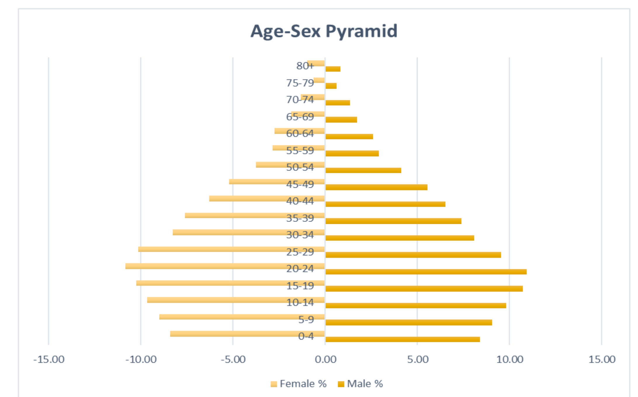
Age-Sex Pyramid
